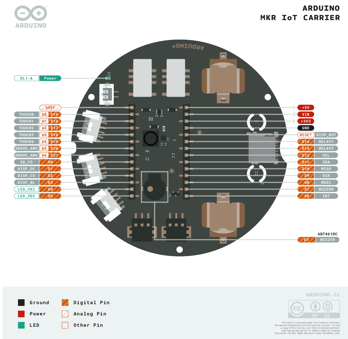
Pinout
